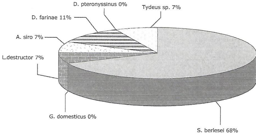
Figure 3. Frequency of human dermatitis caused by environmental mites in autumn-winter in people dealing with poultry houses.
