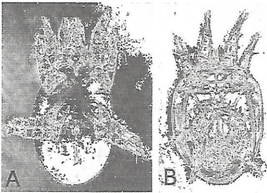
Figure 1. Sancassania berlesei adult (A) and Hypopial deutonymph (Hypopus) (B).
